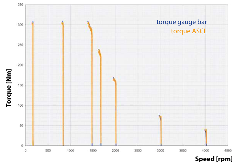
Torque characteristic
